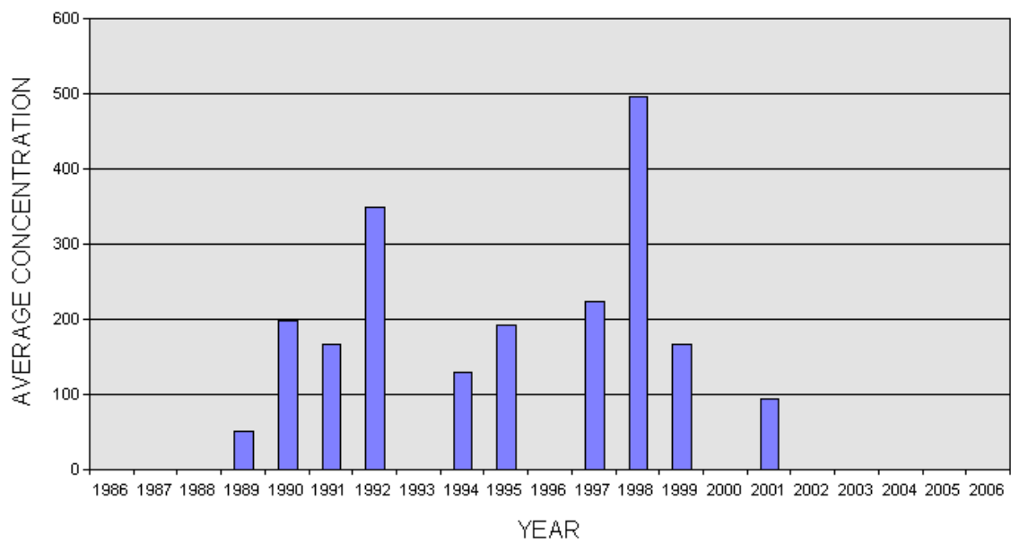
Figure 88. Petroleum aromatic hydrocarbon concentrations (ppb) in bivalve tissue at Sacramento Landing in Tomales Bay in samples taken from 1986 to 2006 (NOAA mussel watch program data).
