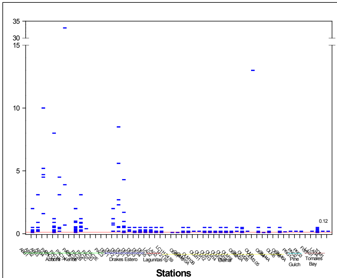
Figure 70. The scatter plot for reactive ammonia ( \text{NH}_4 ) is shown for samples collected from 1999 to 2005 in Point Reyes National Seashore and northern Golden Gate National Recreation Area (N=315)
