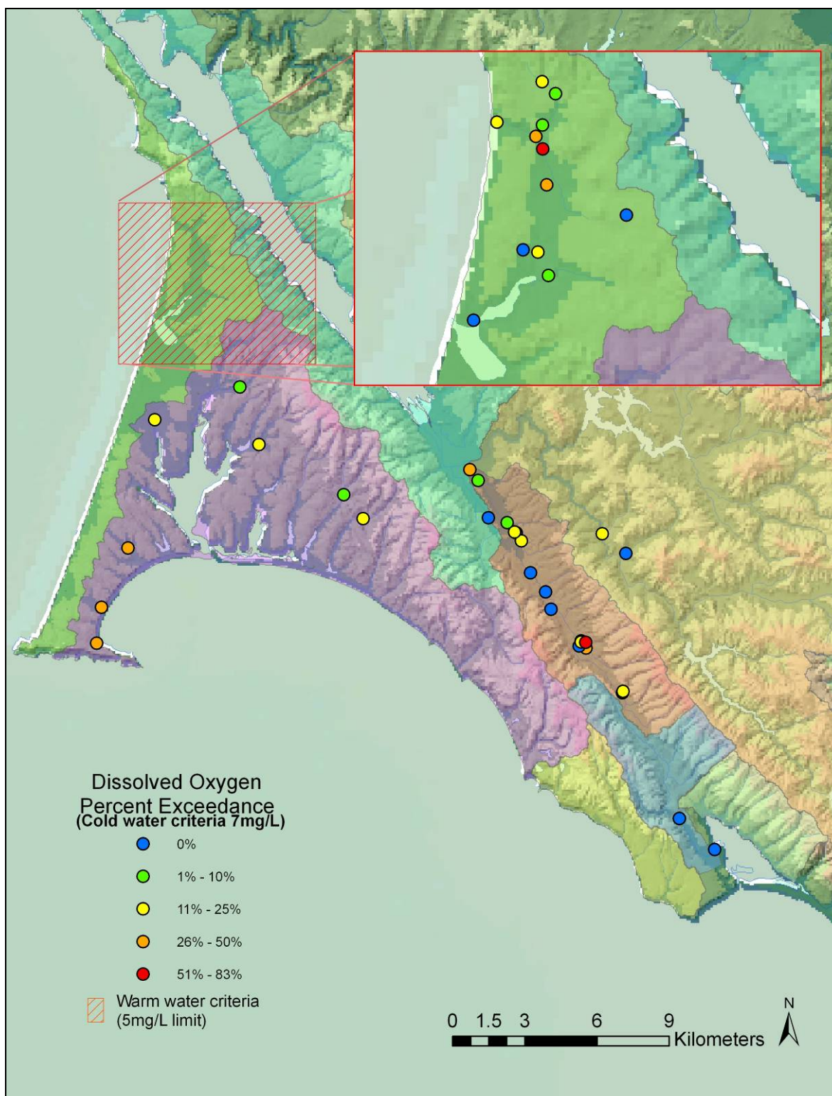
Figure 65. The percent of samples at each water quality sampling location in Point Reyes National Seashore and northern Golden Gate National Recreation Area watersheds where dissolved oxygen minima were below 7 mg/L (ppm) (for cold water sites) or below 5 mg/L (ppm) (for warm water sites).
