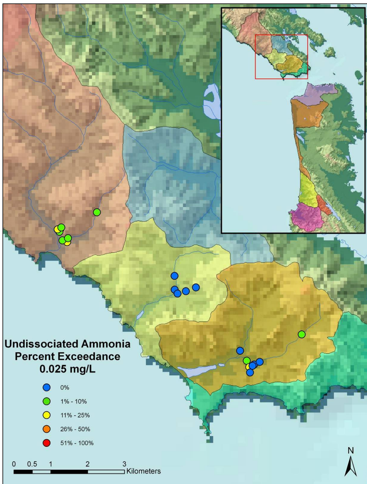
Figure 74. Map of Golden Gate National Recreation Area watersheds illustrates the percentage of water quality samples at each sampling location that exceeded 0.025 mg/L (ppm) of un-ionized (undissociated) ammonia.
