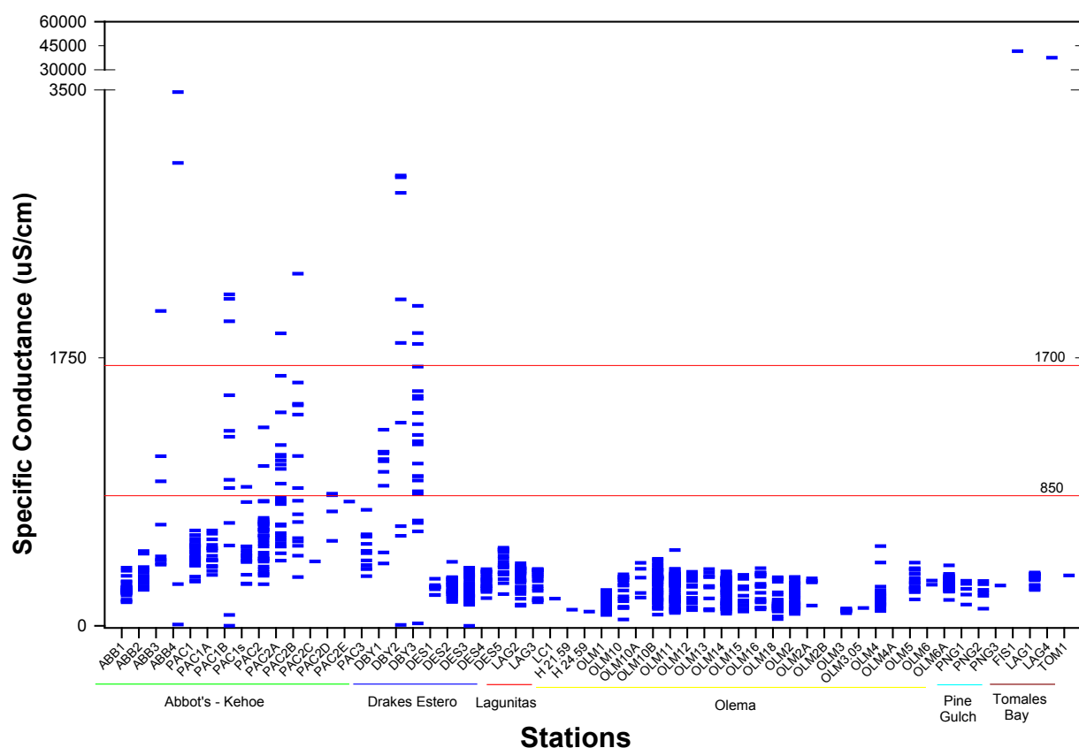
Figure 61. Scatter plot of specific conductance for Point Reyes National Seashore and northern Golden Gate National Recreation Area samples taken from 1999 to 2005, illustrate the samples which are impacted ( >850 \mu\text{S}/\text{cm} ) or toxic to fish ( >1,700 \mu\text{S}/\text{cm} ). High values are exclusively found at estuarine (ABB4, TOM1) and dairy sites, indicating that direct impacts to freshwater fish are limited.
